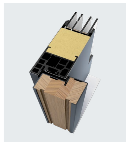
Wood/Steel Frame
